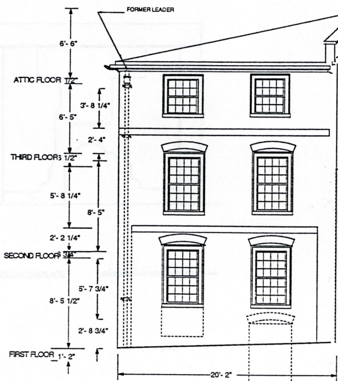
EAST ELEVATION
